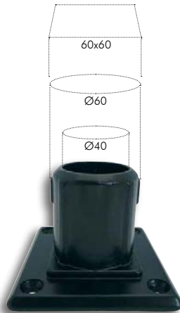
Multibase para Ø40 - Ø60 - 60x60 Ref: MBA4060-*
